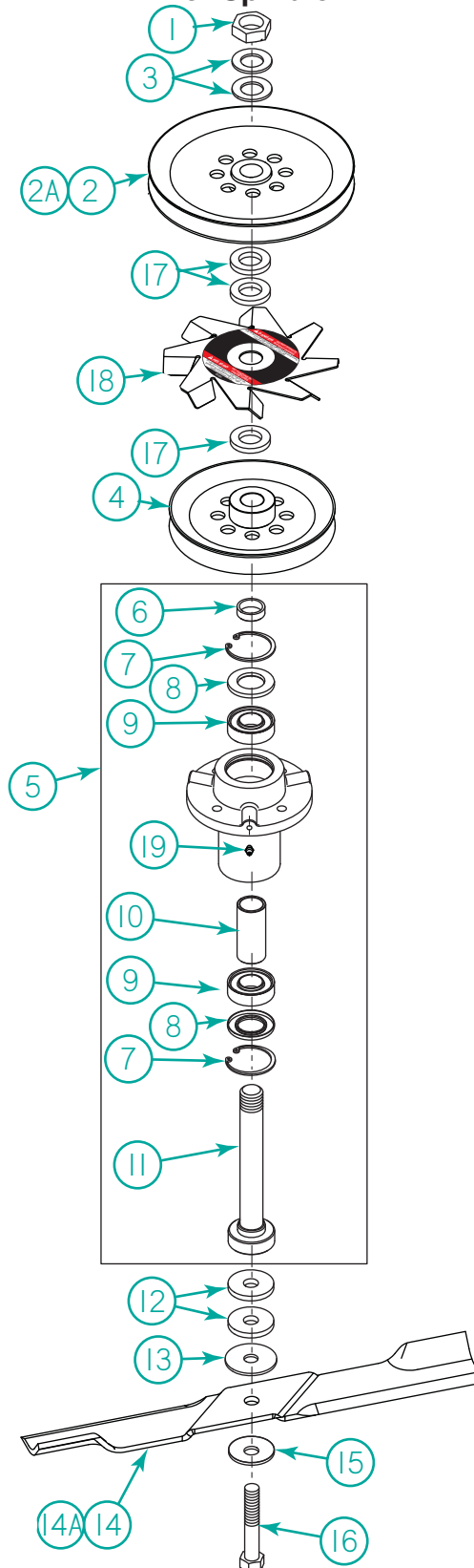
Inner Spindle
