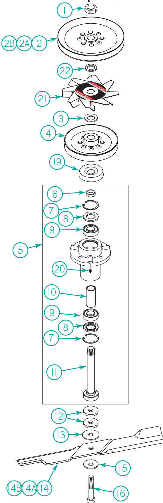
Inner Spindle
